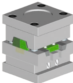
Splits mould KBF 42 AS Type B – using stripper plates
