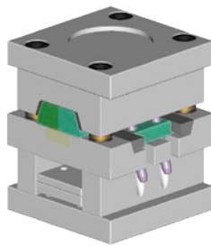
Splits mould KBF 41-AW Type A – using ejector plates
